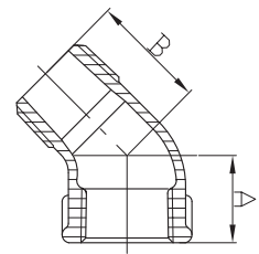
45° Street Elbow
